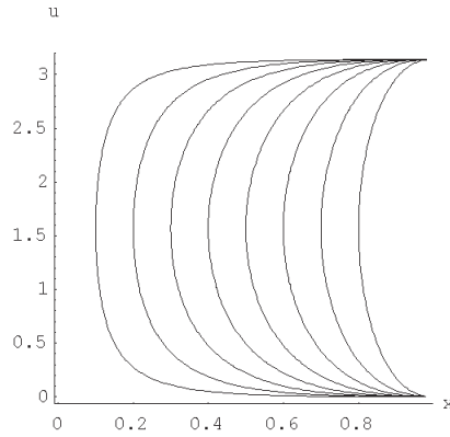
FIGURE 4. Characteristic curves on S_1
