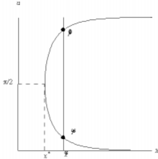
FIGURE 5. Intersection between a characteristic curve and the energy level surface
