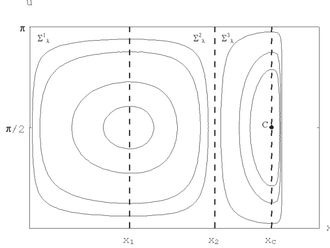
FIGURE 8. Phase portrait of the oscillator for a fixed value of the energy
