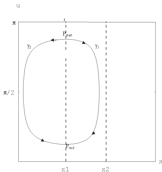
FIGURE 9. Jumping phase trajectories
