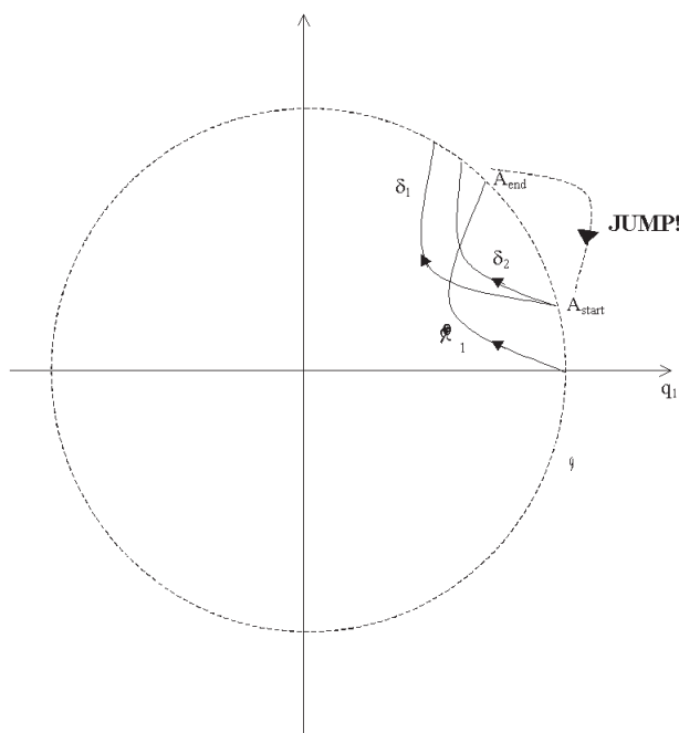
FIGURE 10. Jumping oscillator
