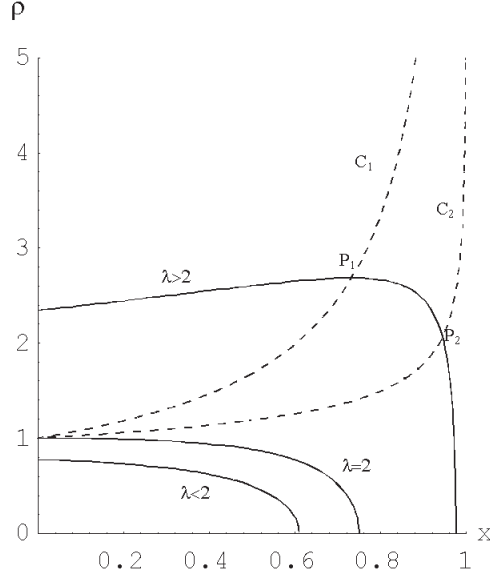
FIGURE 7. Energy level surfaces
