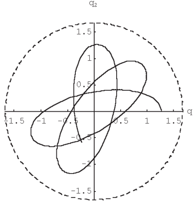
FIGURE 11. Regular precessions
