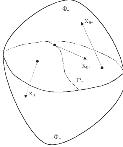
FIGURE 1. In- and out-points
