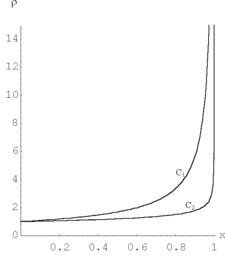
FIGURE 3. Singular surface ( r = r/r_0 )
