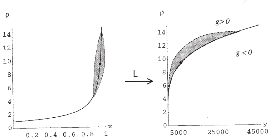
FIGURE 6. Legendre map for the oscillator ( * = r/r_0 )
